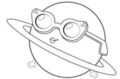
Saturn
