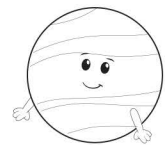
Neptune
